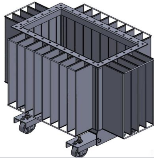
Transformer Tank
