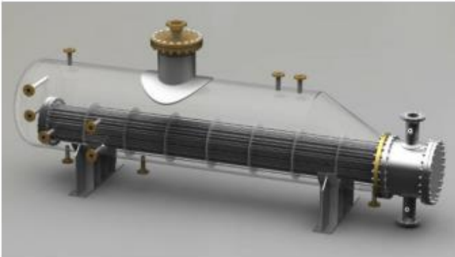
HEAT EXCHANGERS
